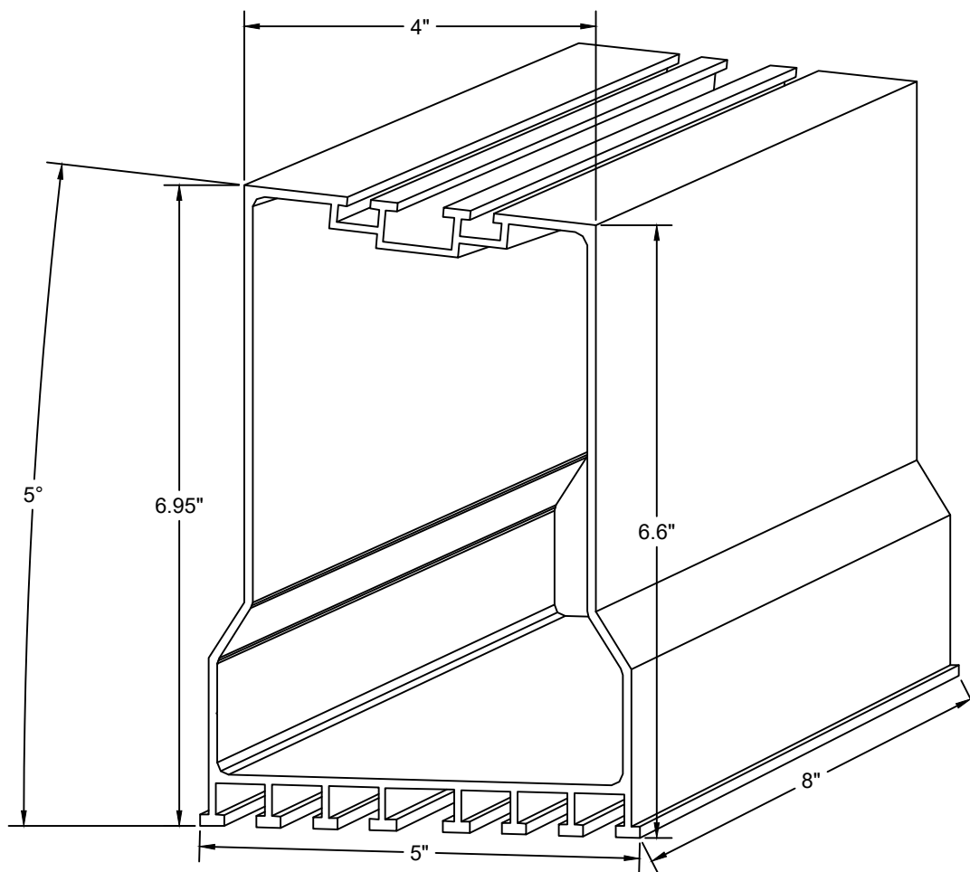
HIGH SOLAR STACK PEDESTAL
