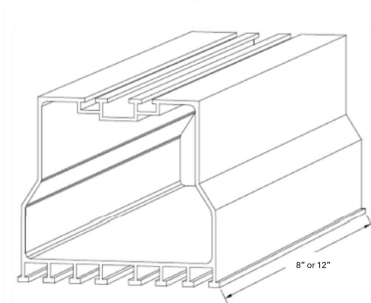
FIGURE 1—SOLAR STACK® SOLAR MOUNTING PEDESTAL
